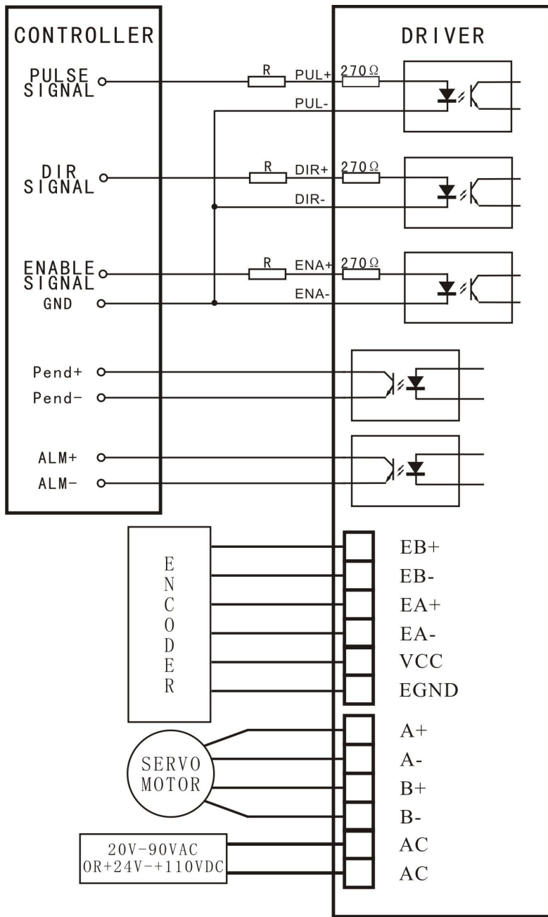
Figure 3: Typical Connection
